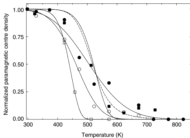
Figure 3. Normalized paramagnetic F^+ -like centre density versus isochronal annealing temperature for YSZ single crystals irradiated with 200 MeV I ions, sample I-14 (line 1, g = 1.998 , open circles), sample I-18 (line 1, g = 1.998 , full circles), and with 200 MeV Au ions, sample AU-5 (line 1, g = 1.998 , open squares), sample AU-11 (line 1, g = 1.998 , full squares). Solid lines are least-squares fits to the first-order kinetics. The dashed line is a least-squares fit to the second-order kinetics for the AU-11 sample.
