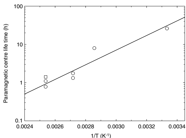
Figure 5. Paramagnetic centre lifetime versus inverse isothermal annealing temperature for YSZ samples (q, r, t) irradiated with 2.0 MeV electrons at the same fluence ( 3.2 \times 10^{18} \text{ cm}^{-2} ) and a sample (f) irradiated with 2.5 MeV electrons and aged at RT [4]: F + -like centres, open circles; hole centres, open squares.
