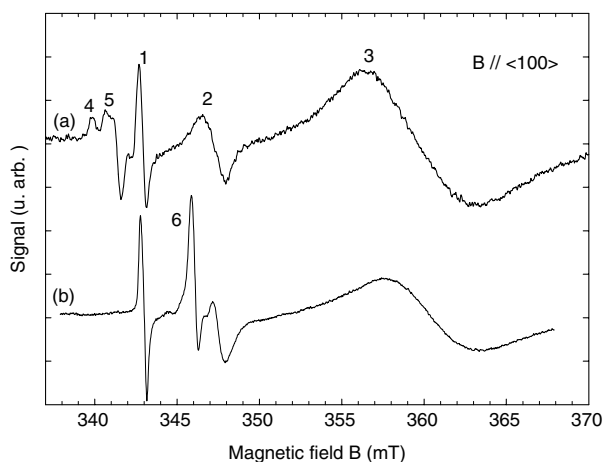
Figure 1. Room-temperature EPR spectrum with B \parallel \langle 100 \rangle of an as-received YSZ(100) single crystal irradiated with 2.0 MeV electrons (sample q) (a); and a vacuum-annealed reduced YSZ (100) single crystal irradiated with 100 MeV C ions (sample C-20) and annealed in air at 873 K [4] (b).
