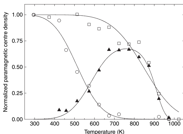
Figure 6. Normalized paramagnetic centre density versus isochronal annealing temperature for a YSZ single crystal (sample C-20) irradiated with 100 MeV C ions at a fluence of 9.3 \times 10^{14} \text{ cm}^{-2} [4]: F + -like centres (open circles), T centres (open squares), new centres (full triangles). Solid lines are least-squares fits to first-order kinetics modelling.
