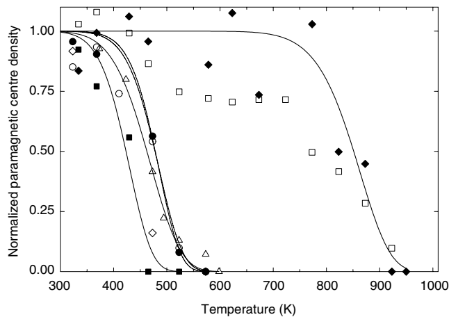
Figure 2. Normalized paramagnetic centre density versus isochronal annealing temperature for electron-irradiated YSZ single crystals: sample e (1.0 MeV), T centres (line 3, g = 1.904 , open triangles); sample j (1.0 MeV), F^+ -like centres (line 1, g = 1.998 , full squares), T centres (line 3, g = 1.904 , open squares), T centre satellite ( g = 1.97 , full diamonds); sample s (2.0 MeV), F^+ -like centres (line 2, g = 1.973 , full circles), T centres (line 3, g = 1.904 , open circles), hole centres (line 5, g = 2.007 , open diamonds). Lines are least-squares fits to the first-order kinetics.
